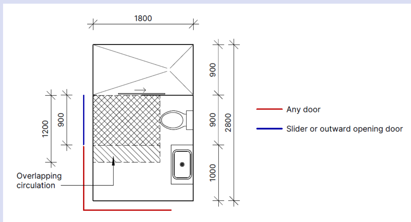
Figure C.5 Bathroom layout – 5.04 m 2 (dimensions in mm)
