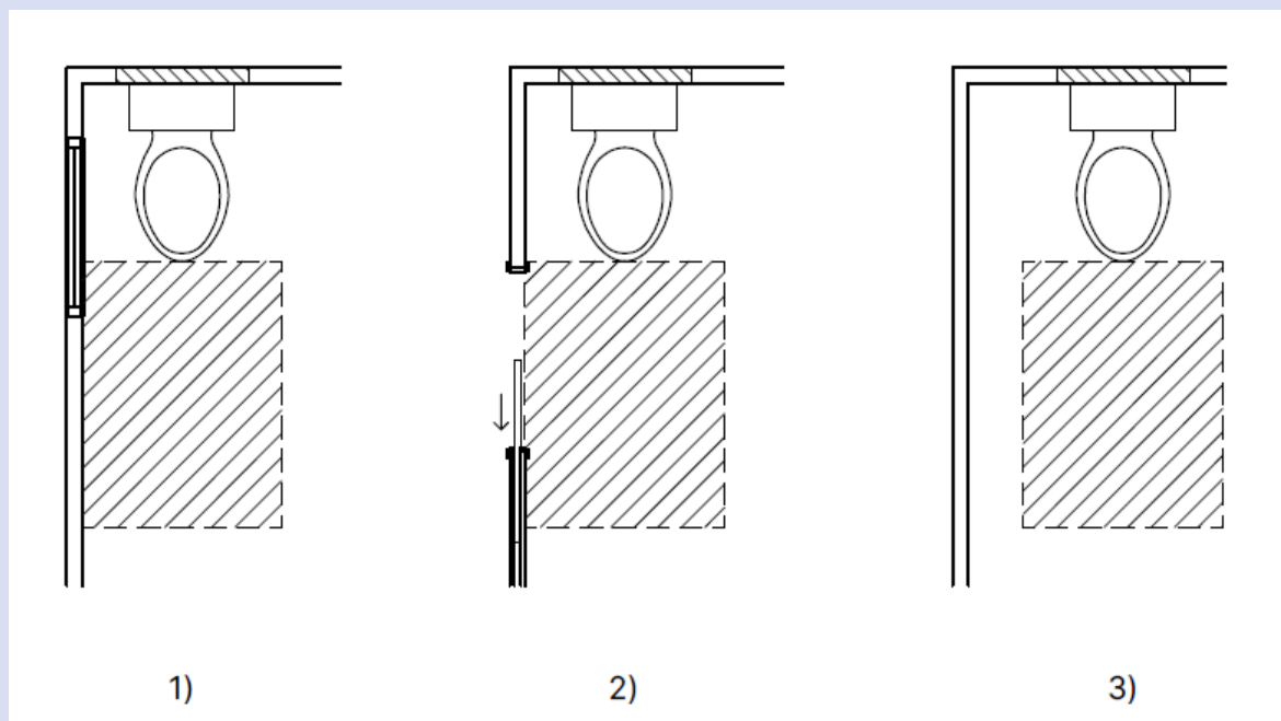
Figure 8.2 Examples of reinforcing behind the toilet pan
