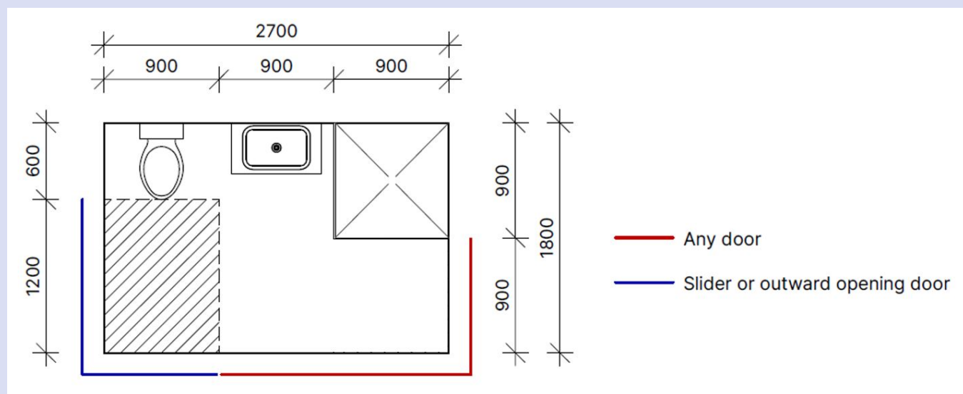
Figure C.2 Bathroom layout – 4.86 m 2 (dimensions in mm)
